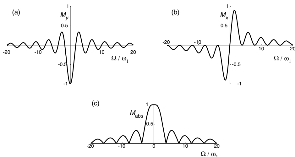
Fig. 3.26 Plots of the magnetization produced by a pulse as a function of the offset. The pulse length has been adjusted so that on resonance the flip angle is 90^\circ . The horizontal axes of the plots is the offset expressed as a ratio of the RF field strength, \omega_1 ; the equilibrium magnetization has been assumed to be of size 1.
